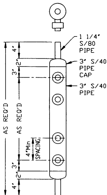
TYPE LEVEL INDICATOR COLUMN FOR H.P. RECEIVER
