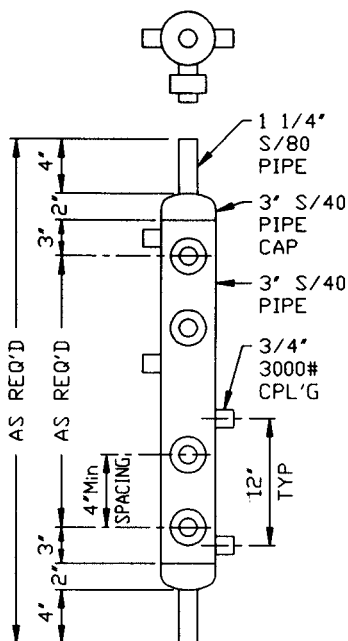
TYPE LEVEL INDICATOR COLUMN FOR VESSELS WITH FLOAT SWITCHES
