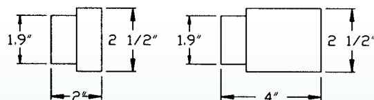
TYPE LEVEL INDICATOR COLUMN FOR VESSELS WITH VARI-LEVEL CONTROLS
