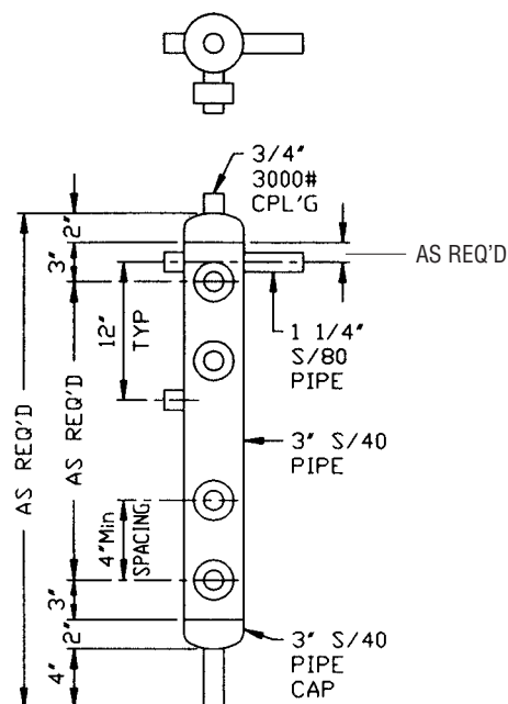
TYPE LEVEL INDICATOR COLUMN FOR VESSELS WITH VARI-LEVEL CONTROLS
