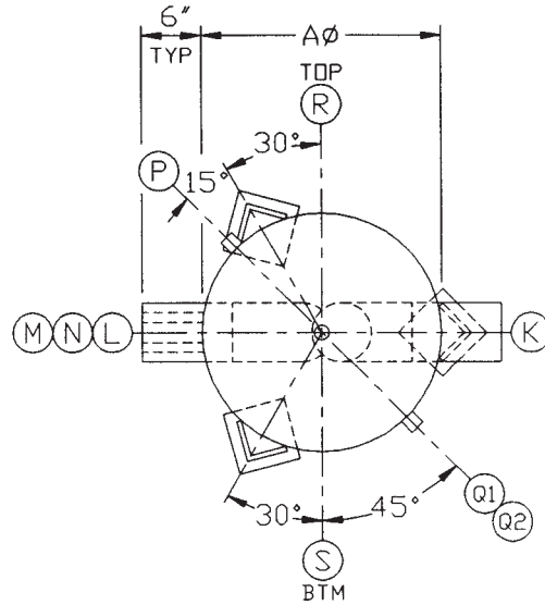
VIEW "Z-Z"
